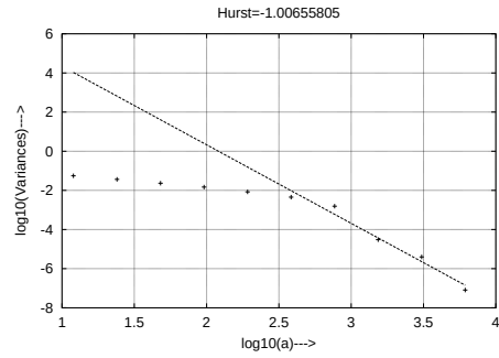
e) Snowboard with Comm with 128 kbps target bit rate
