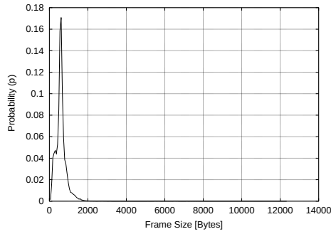
b) Oprah w/o Comm with low quality
