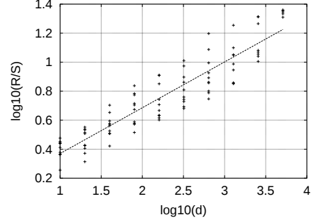
d) Star Wars IV with 256 kbps target bit rate, H=0.657
