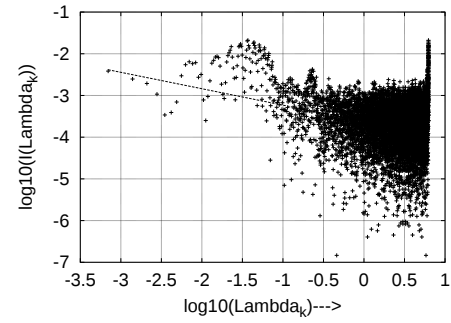
e) Jurassic Park I with 128 kbps target bit rate, H=0.696
